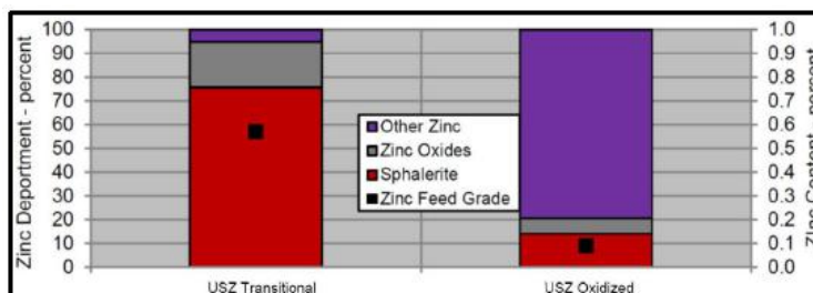
Figure 13-3 Deportment of Zinc for the USZ Oxidized and USZ Transitional Composite Samples
