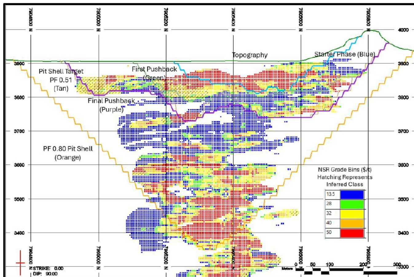
Figure 16-8 Pit Designs, NS Section View, 593150E
