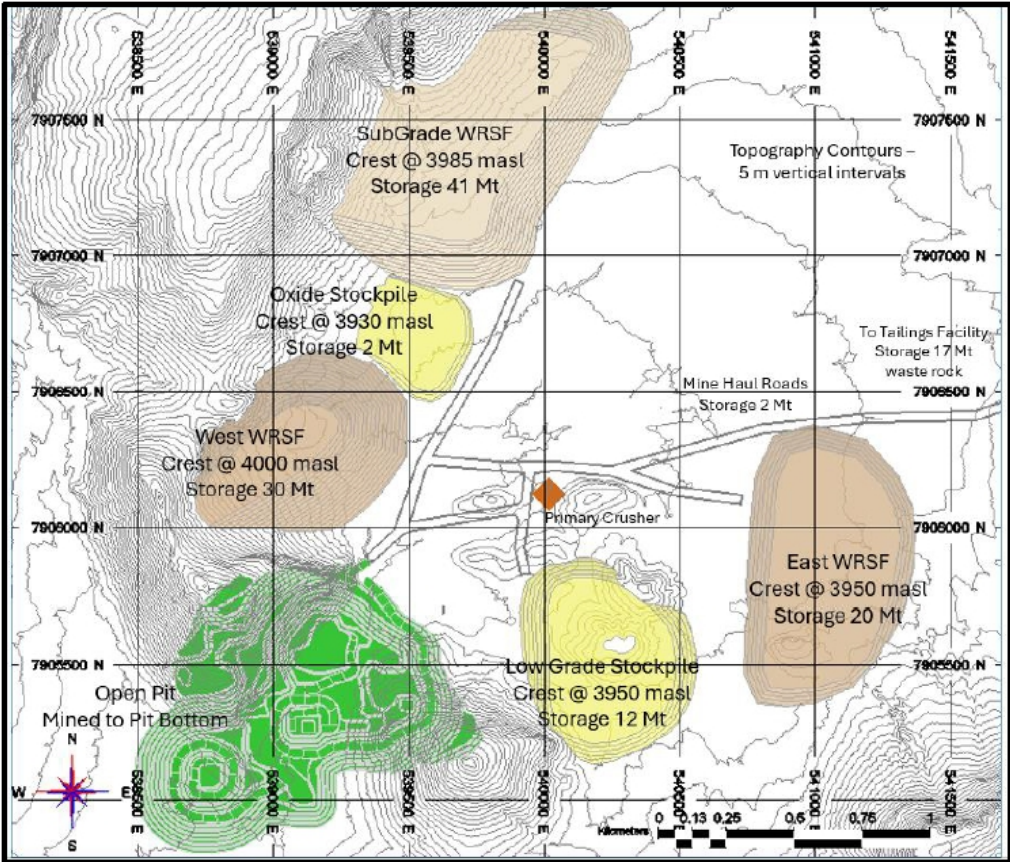
Figure 16-16 End of Period Production Schedule, Year 13
