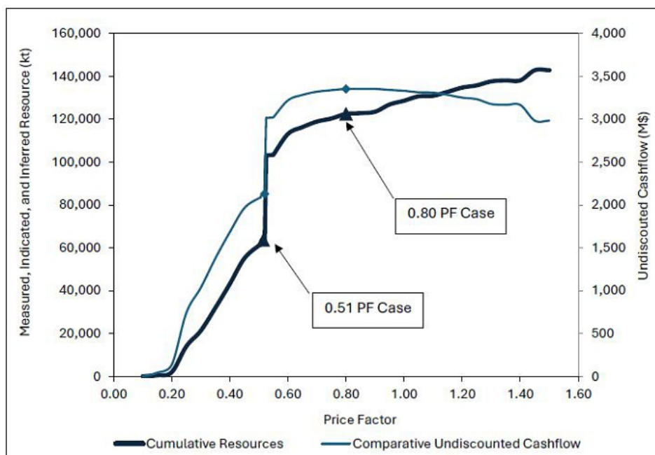
Figure 16-3 Pseudoflow Pit Shell Resource Contents by Case
