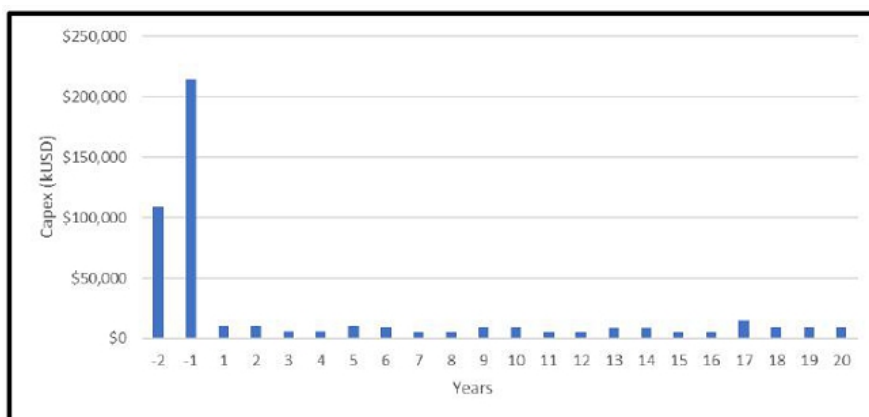
Figure 21-1 CAPEX Distribution
