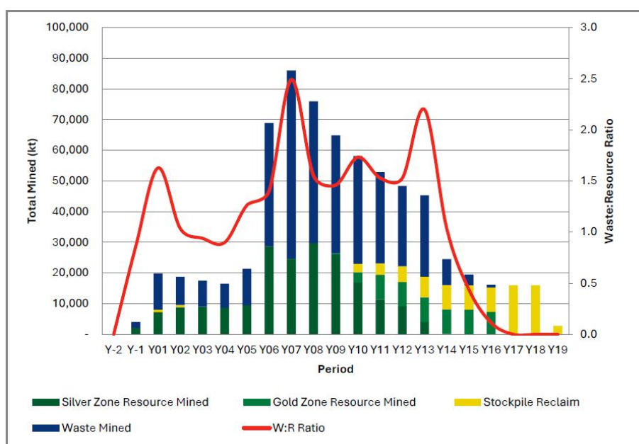
Figure 24-6 Alternate Production Scenario Mine Production Summary
