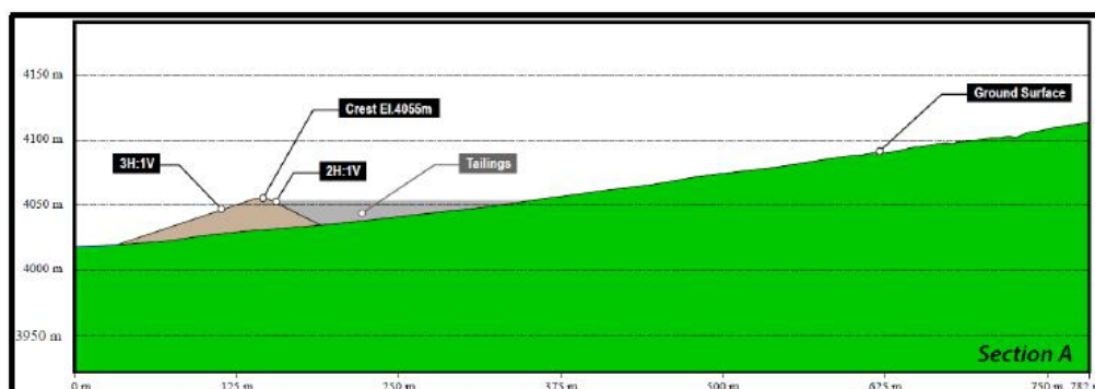
Figure 18-6 Conventional TSF Option 1 – Maximum Cross-Section
