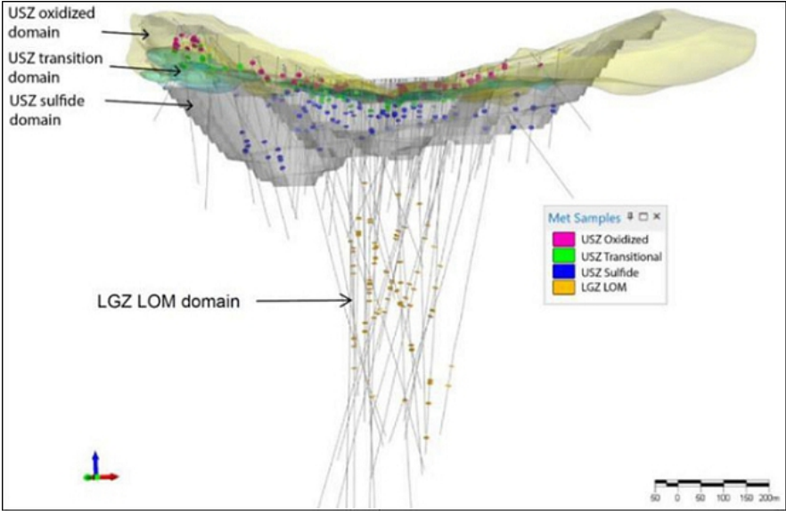
Figure 13-1 Locations of the Intervals Selected for the Metallurgical Samples
