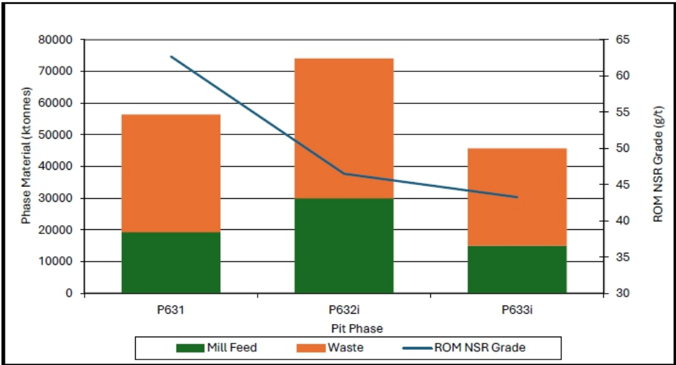
Figure 16-4 Designed Open Pit Contents
