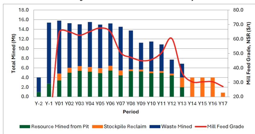
Figure 1-1 Mine Production Schedule Summary
