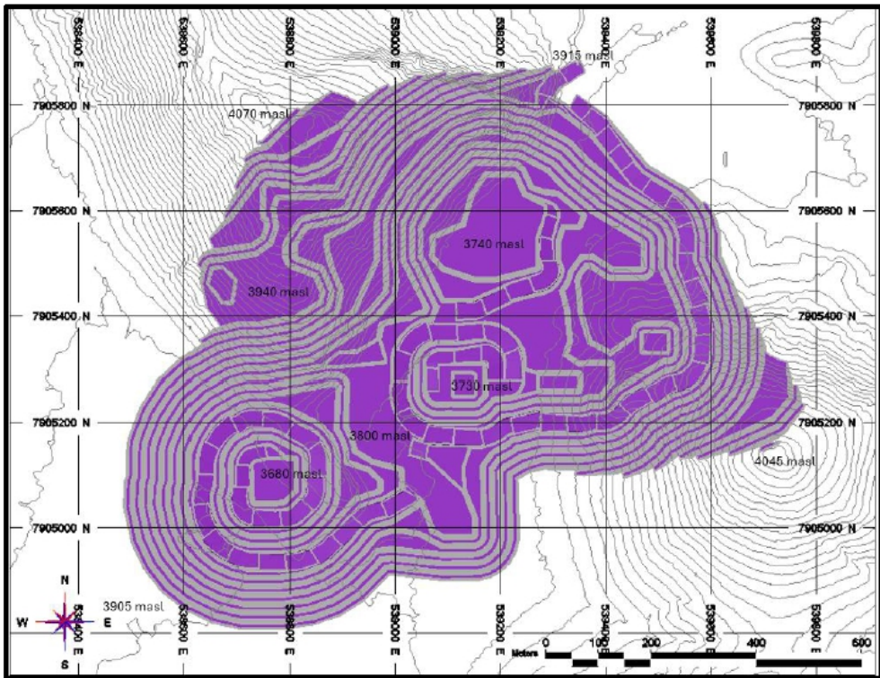
Figure 16-5 Ultimate Pit Design, P633
