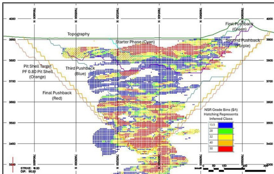
Figure 24-2 Alternate Pit Designs, NS Section View, 593150E
