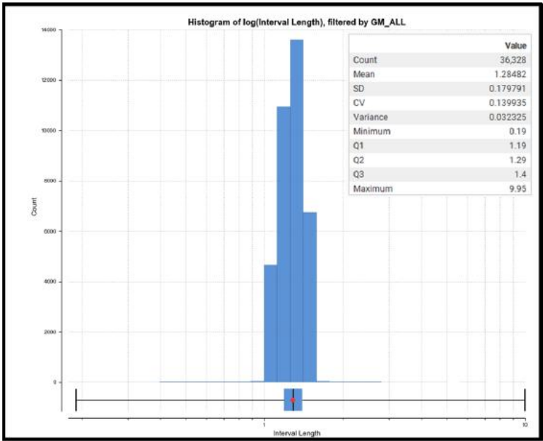
Figure 14-3 Length Histogram for Raw Assay Intervals
