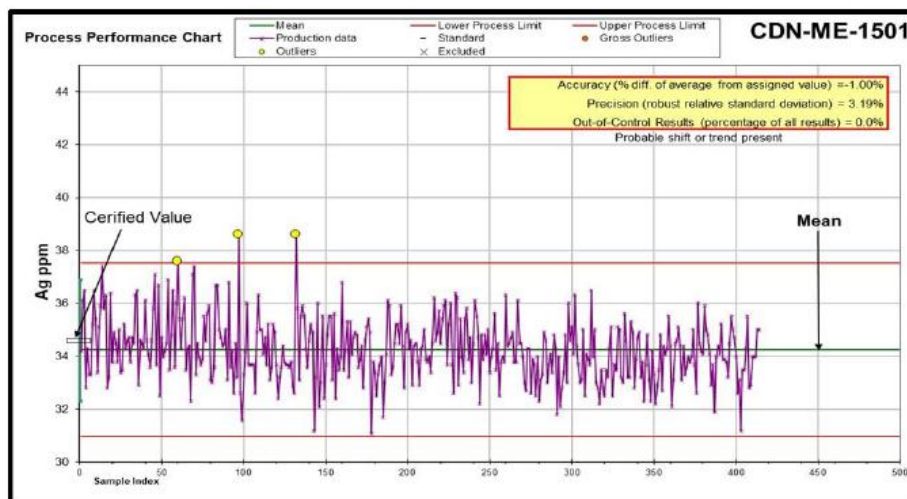
Figure 11-4 Control Chart for CDN-ME-1501 (Ag) (July 2021 – November 2022)
