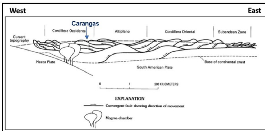
Figure 8-1 Schematic Cross-Section of Bolivia Region
