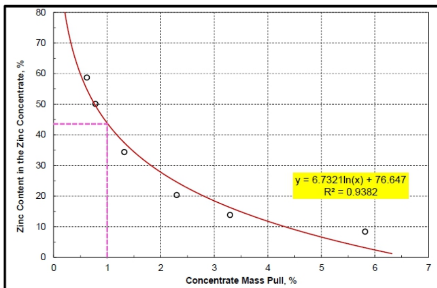
Figure 13-14 Zinc Content in the Concentrate for the USZ LOM Composite Sample
