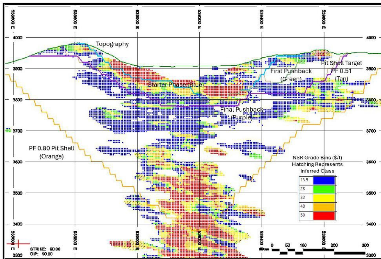
Figure 16-7 Pit Designs, EW Section View, 7905400N
