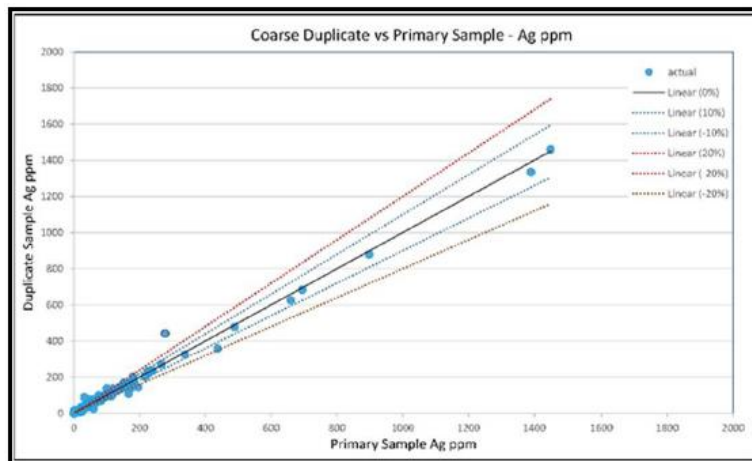
Figure 11-9 Coarse Duplicate Precision Scatterplot – Silver Assays
