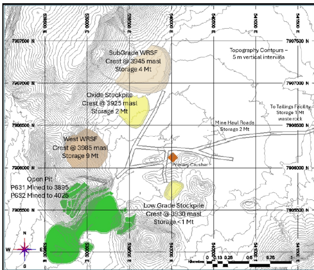
Figure 16-12 End of Period Mine Production Schedule, Year -1
