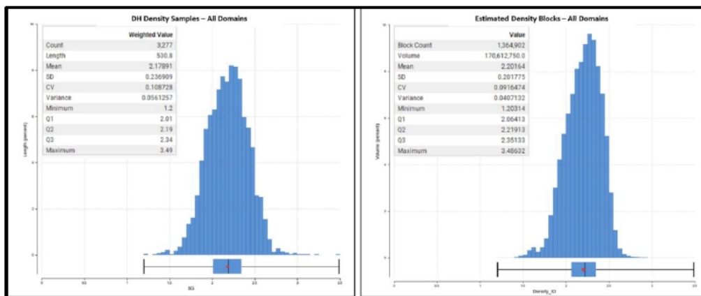
Figure 14-4 Estimation Density Histogram Validation
