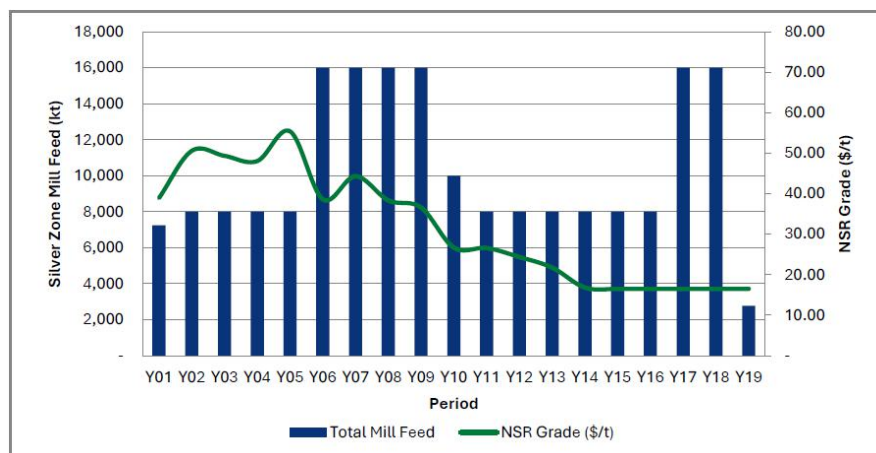
Figure 24-4 Alternate Production Scenario: Silver Zone Mill Feed
