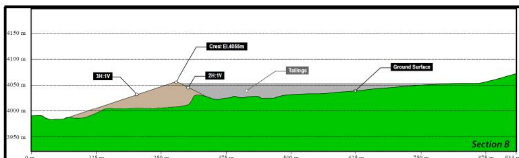
Figure 18-5 Conventional TSF NE – Cross-Section
