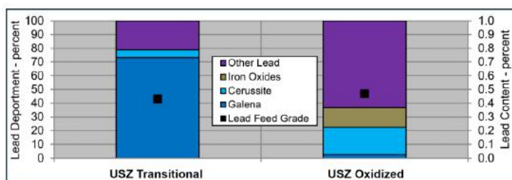
Figure 13-2 Deportment of Lead for the USZ Oxidized and USZ Transitional Composite Samples
