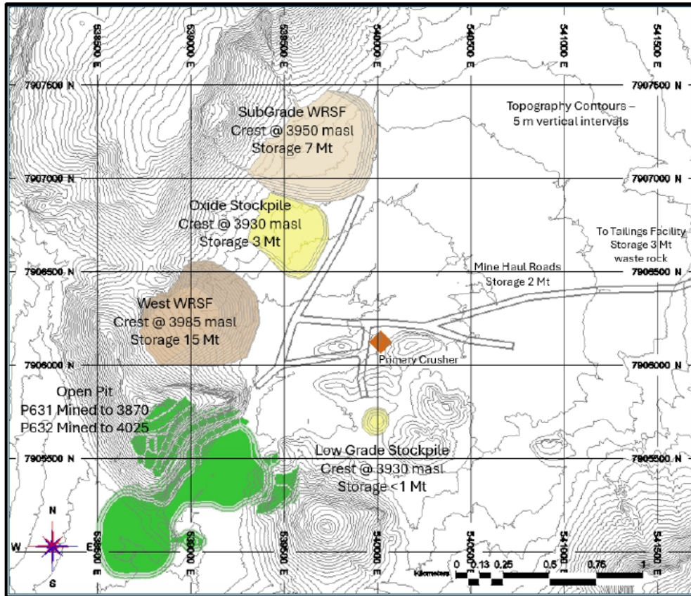
Figure 16-13 End of Period Mine Production Schedule, Year 1
