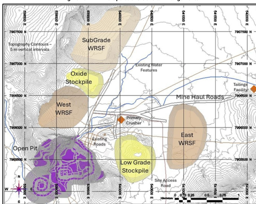
Figure 16-1 Mine Operations General Arrangements
