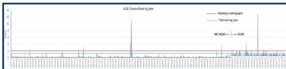
Figure 11-5 Control Chart for Coarse Blank Samples
