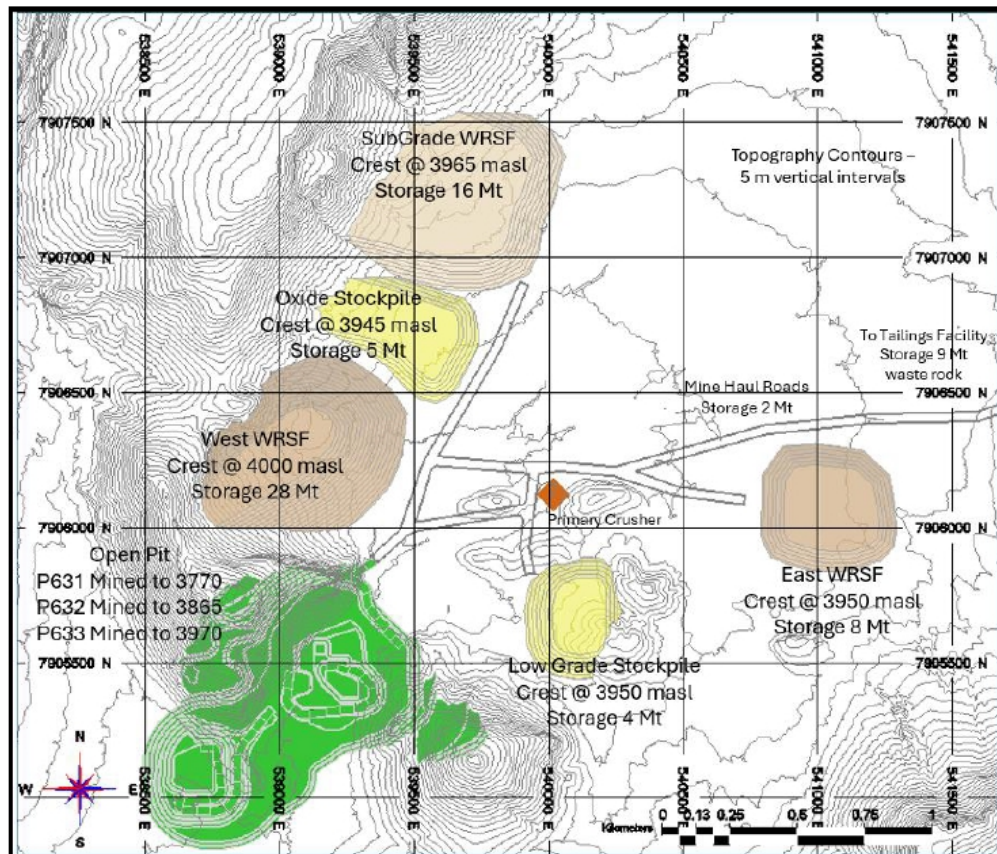
Figure 16-15 End of Period Production Schedule, Year 5
